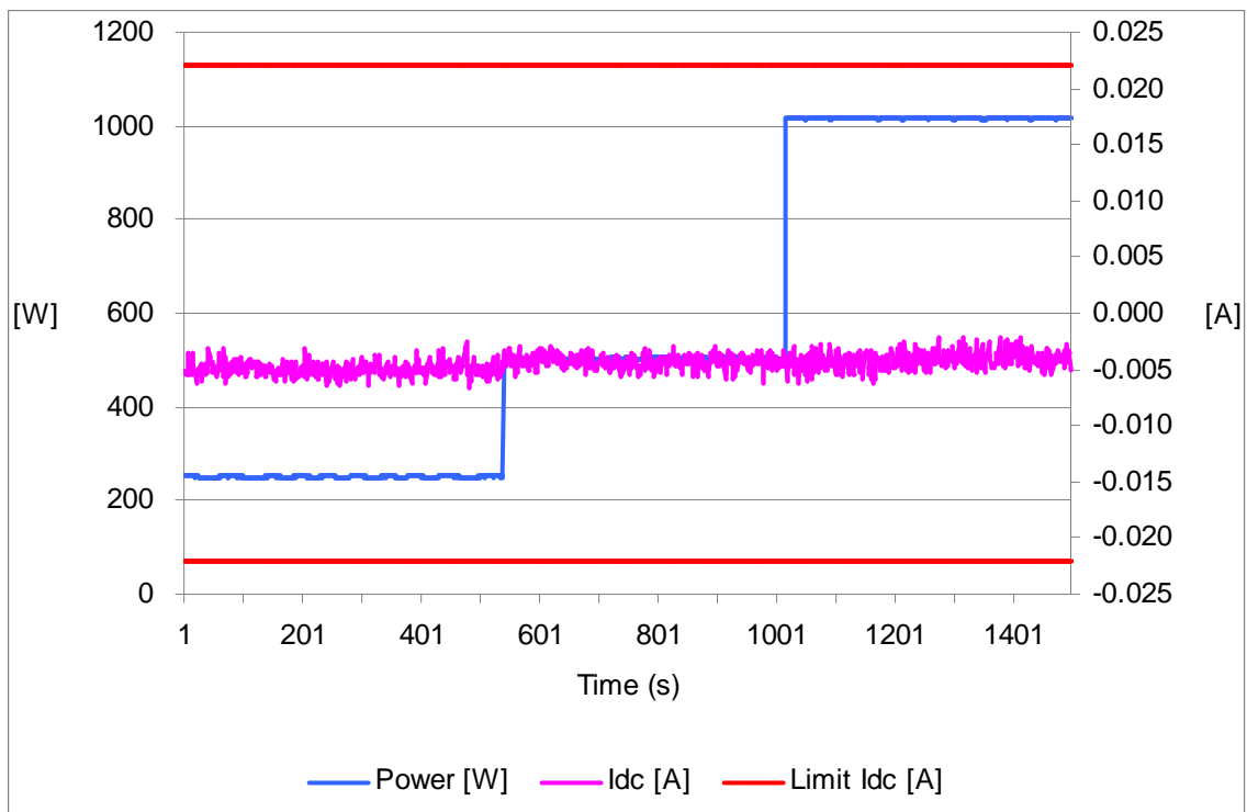
Diagram of permanent dc-injection: SOFAR 1100TL
